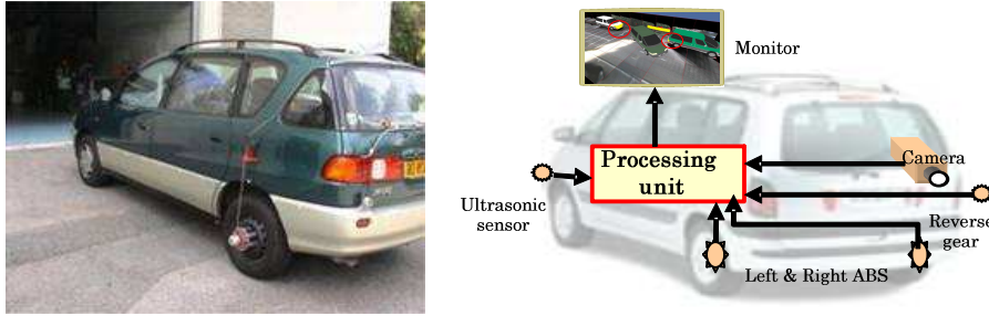
Figure 2: Prototype setup.
